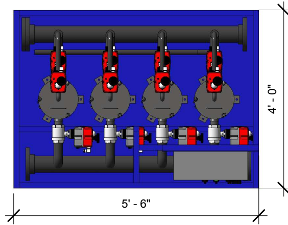
① Top \frac{1}{2}'' = 1'-0''
